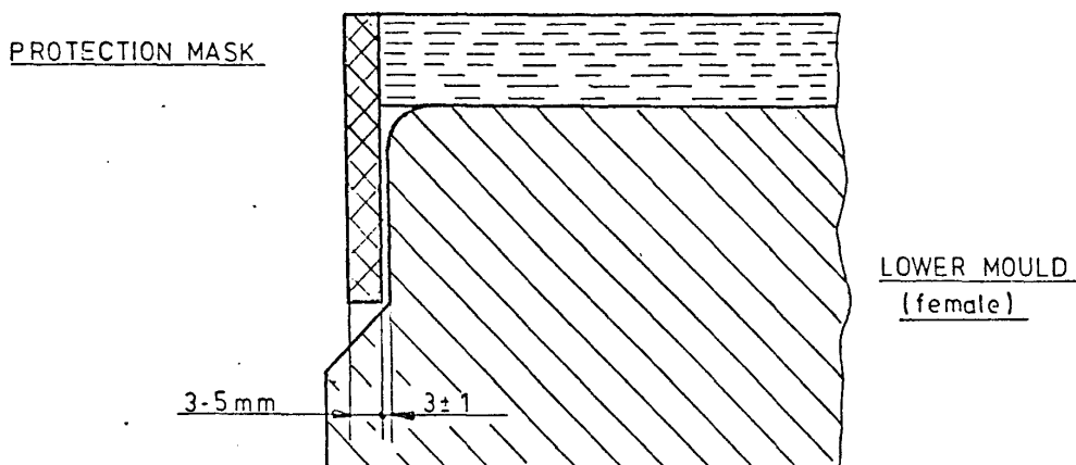
Figure 3: Preferred mould venting design.
