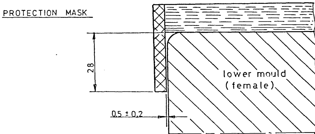
Figure 2: Adapted mould vent design for existing moulds.
